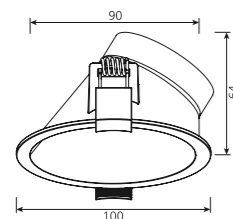
ASYMMETRICAL TRIM Ø95
