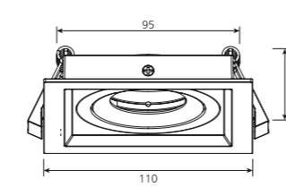
OVAL HOLE TRIM Ø80
